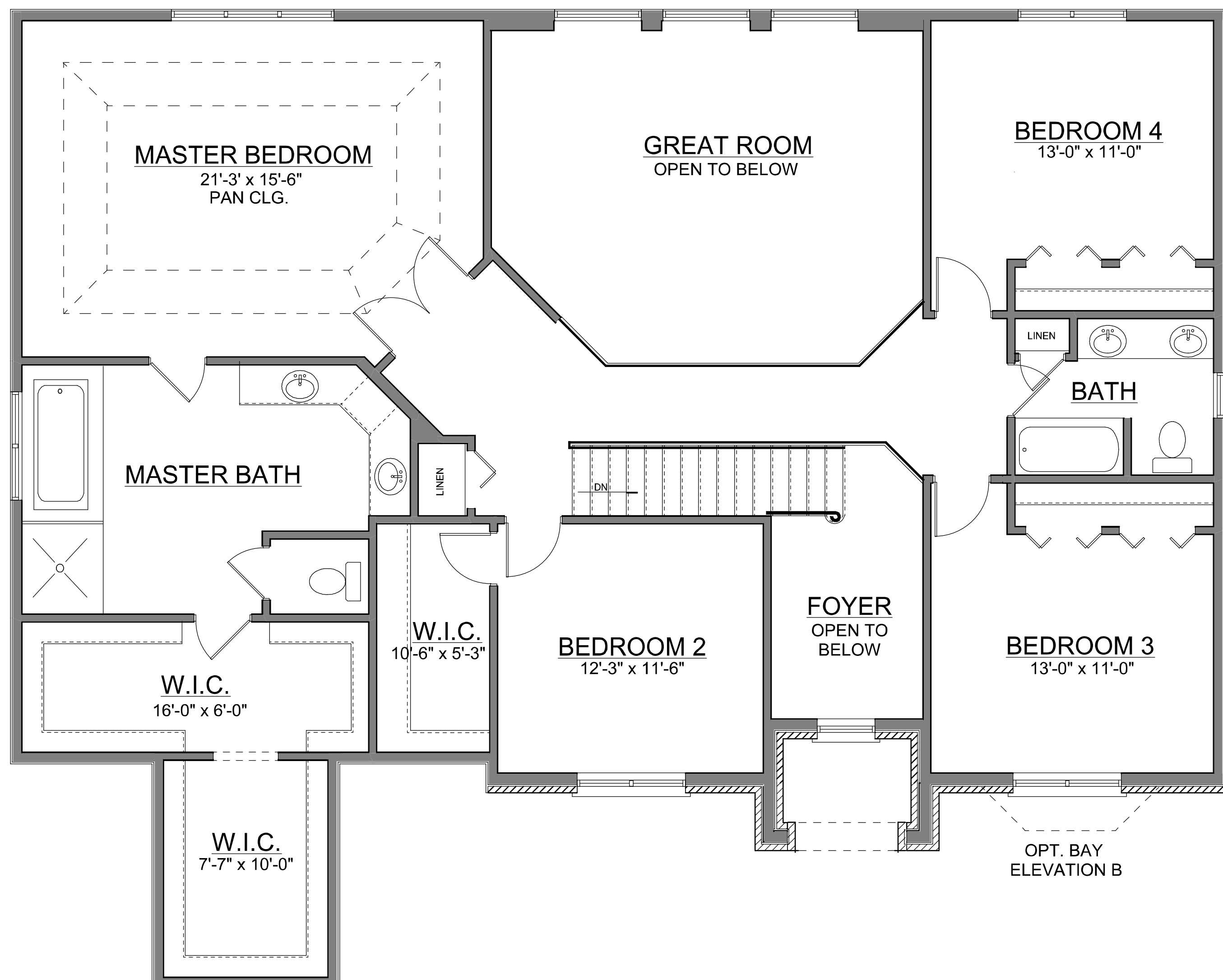
SECOND FLOOR PLAN 2-BATH OPT.
